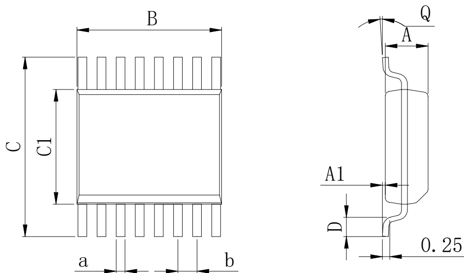
Dimensions In Millimeters(QSOP-16)
